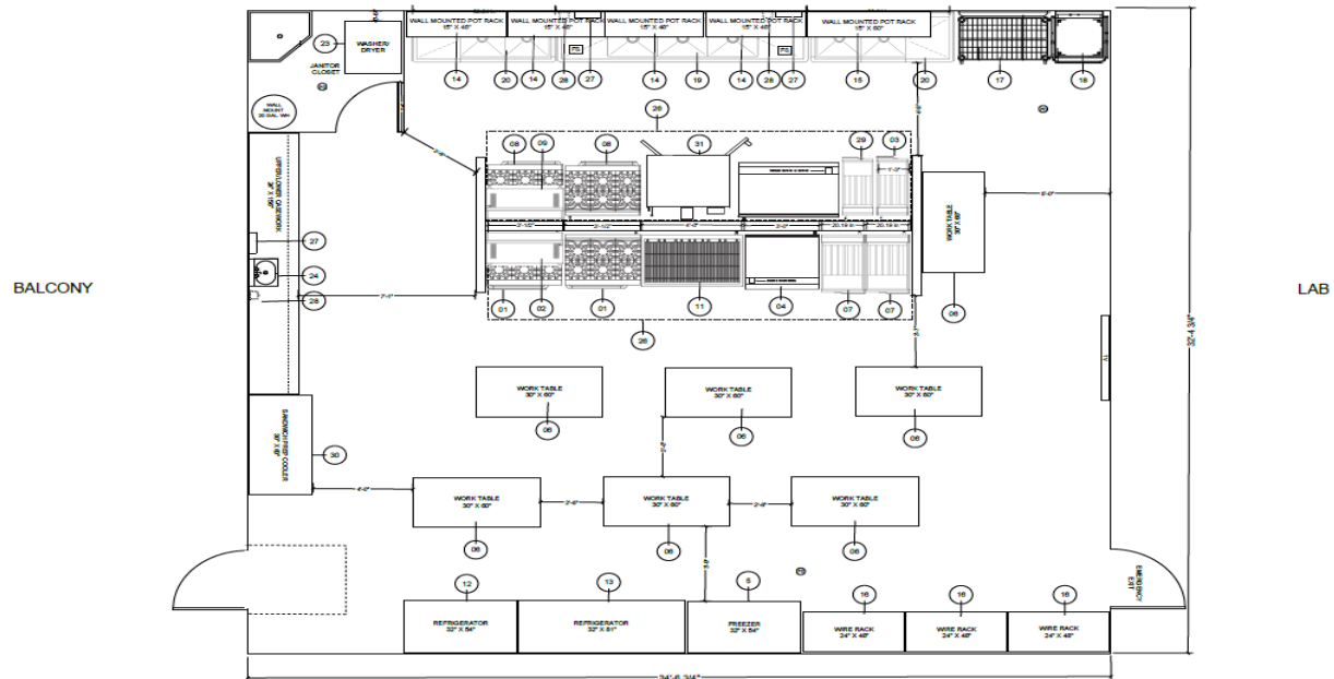
Initial concept of Culinary equipment layout
